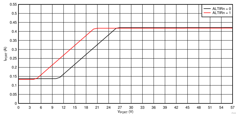
Figure 9-81. Inrush Foldback Curves, I_{PORT} vs V_{PORT}
