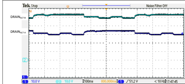
Figure 10-12. 4-Pair Low Resistance (11kΩ) Detection Signature
