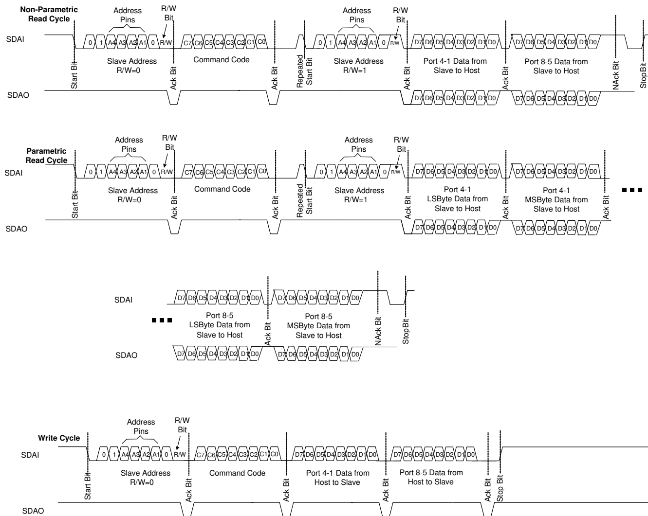
Figure 9-7. I²C interface Read and Write Protocol – Configuration B
