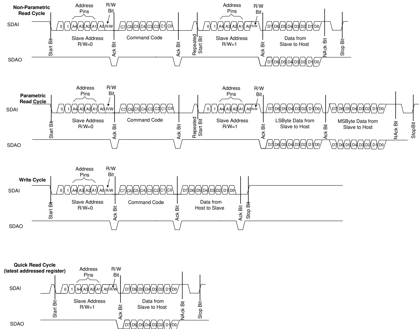
Figure 9-6. I²C interface Read and Write Protocol – Configuration A
