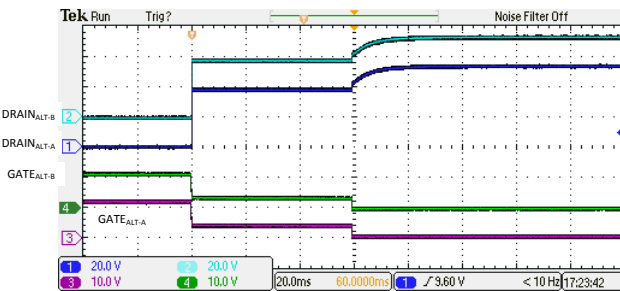
Figure 10-6. 4-Pair I_{LIM} Foldback and Turn Off
