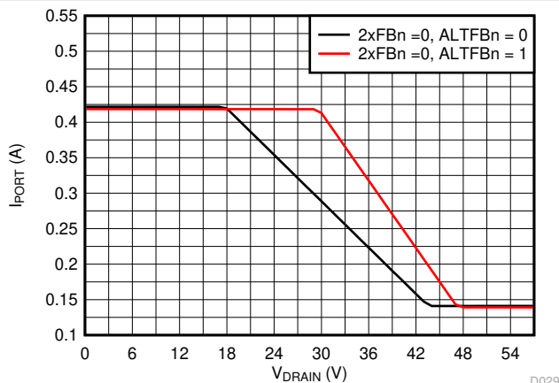
Figure 7-29. 1x Mode (2xFBn = 0) Current Foldback vs Drain Voltage
