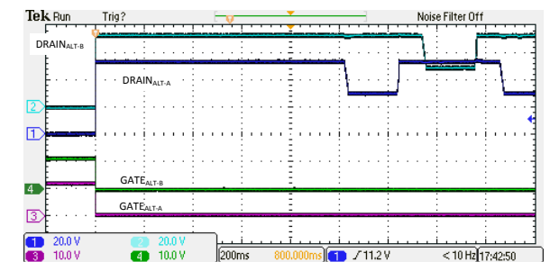
Figure 10-8. 4-Pair Backoff Due to 4PPCut Fault
