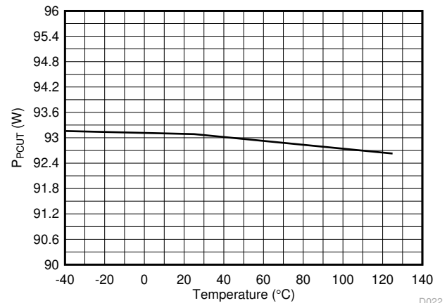
Figure 7-22. 4-Pair PCut Threshold (90W) vs Temperature
