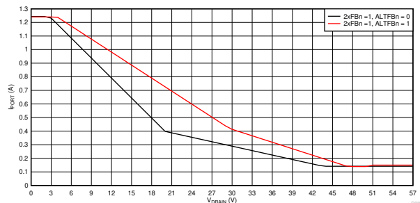
Figure 9-57. 2x Mode (2xFBn = 1) Foldback Curves, I_{PORT} vs V_{DRAIN}
