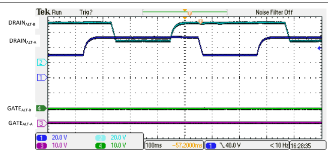
Figure 10-11. 4-Pair Open Circuit Detection Signature
