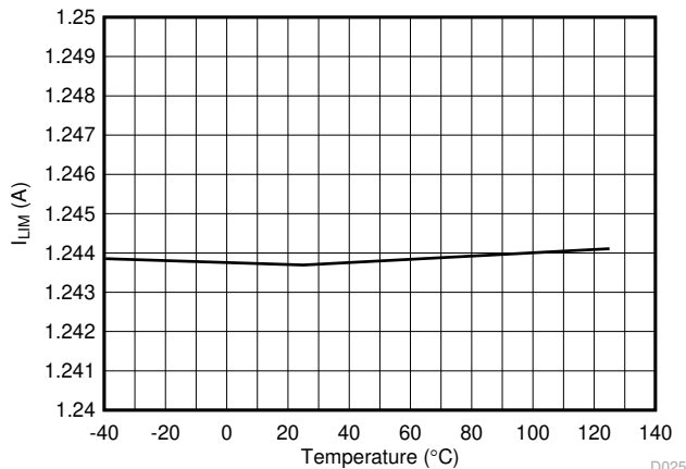
Figure 7-25. 2x Mode (2xFBn = 1) Current Limit vs Temperature
