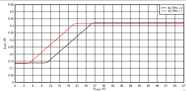
Figure 9-2. Foldback During Inrush (at Port Turn-On): I_{LIM} vs V_{port}
