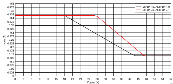
Figure 9-79. 1x Mode (2xFBn = 0) Foldback Curves, I_{PORT} vs V_{DRAIN}
