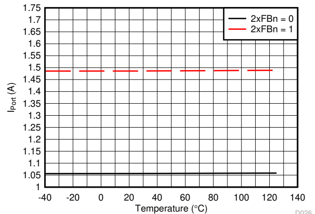
Figure 7-26. I_{\text{SHORT}} Threshold vs Temperature
