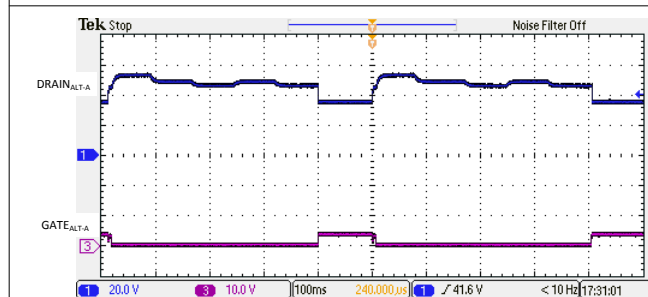
Figure 10-14. 2-Pair Semiauto Mode Discovery with a Valid Class 0-3 Load
