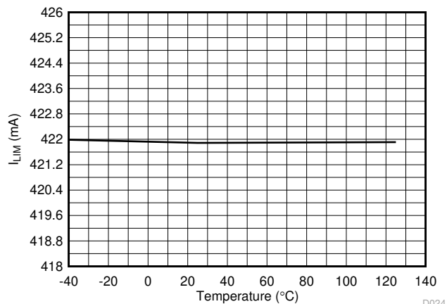
Figure 7-24. 1x Mode (2xFBn = 0) Current Limit vs Temperature
