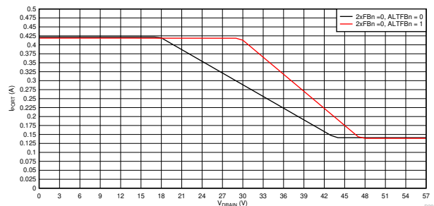
Figure 9-56. 1x Mode (2xFBn = 0) Foldback Curves, I_{PORT} vs V_{DRAIN}
