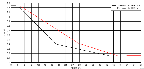
Figure 9-80. 2x Mode (2xFBn = 1) Foldback Curves, I_{PORT} vs V_{DRAIN}
