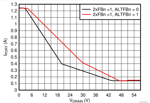
Figure 7-30. 2x Mode (2xFBn = 1) Current Foldback vs Drain Voltage
