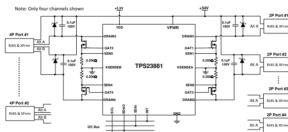
Simplified Schematic
