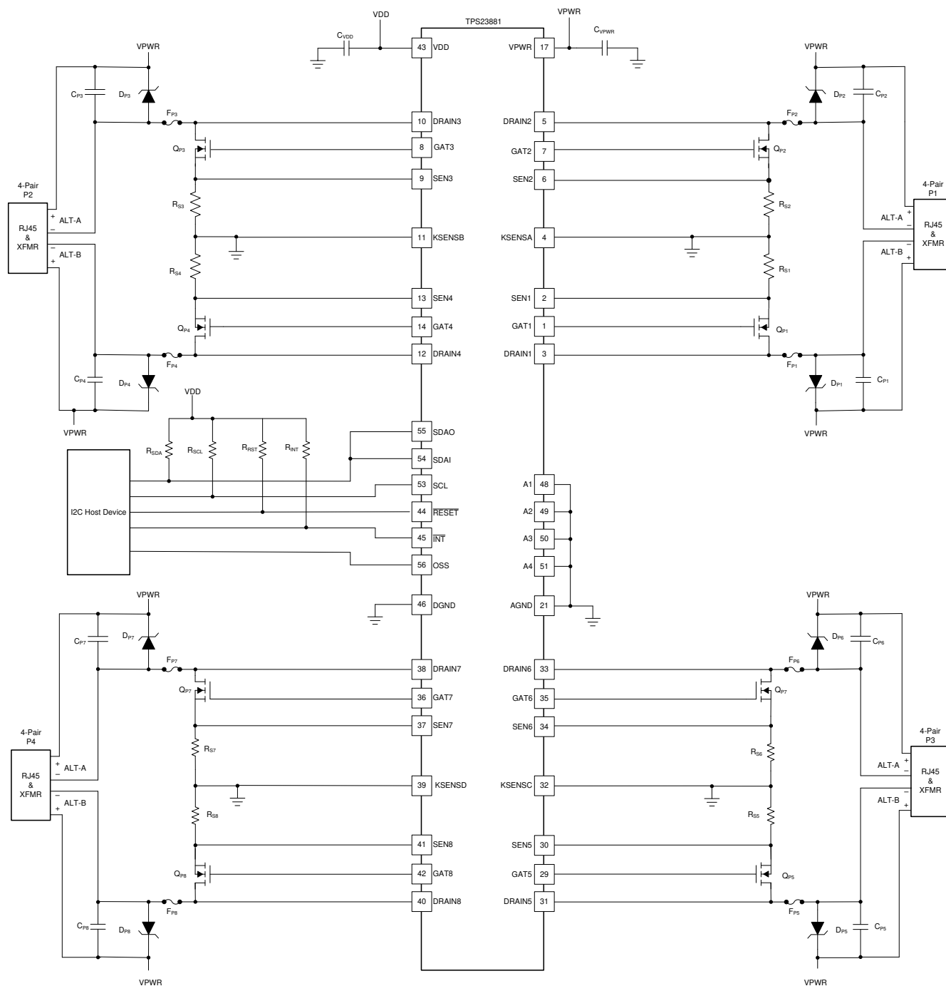
Figure 10-2. Four 4-Pair Port Application
