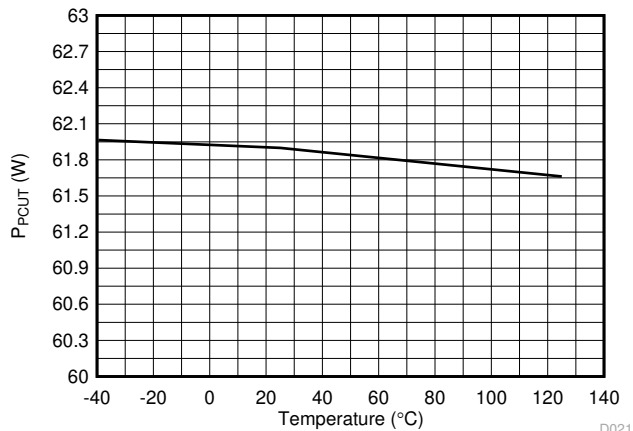
Figure 7-21. 4-Pair PCut Threshold (60W) vs Temperature
