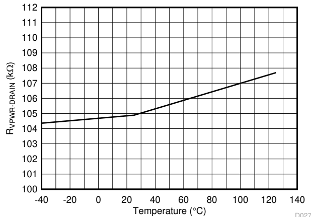
Figure 7-27. R_{\text{OFF}} (VPWR to DRAIN) vs Temperature
