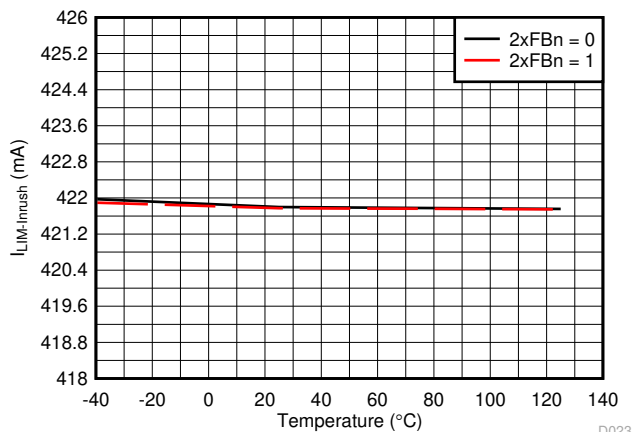
Figure 7-23. Inrush Current Limit vs Temperature
