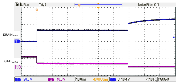
Figure 10-4. 2-Pair I_{LIM} Foldback and Turn-Off
